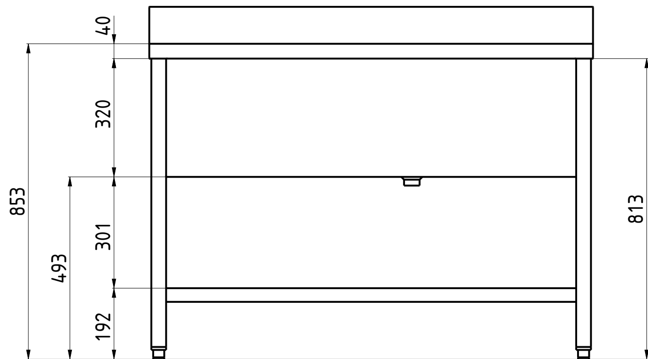
FRONT VIEW 1:10
