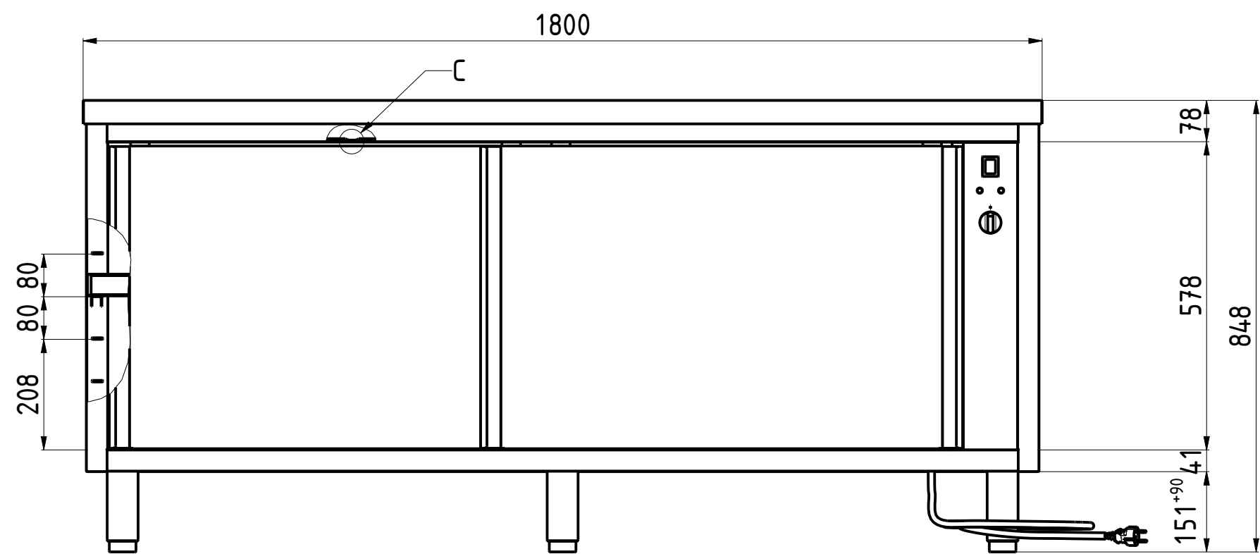
FRONT VIEW B-B C-C 1:10
