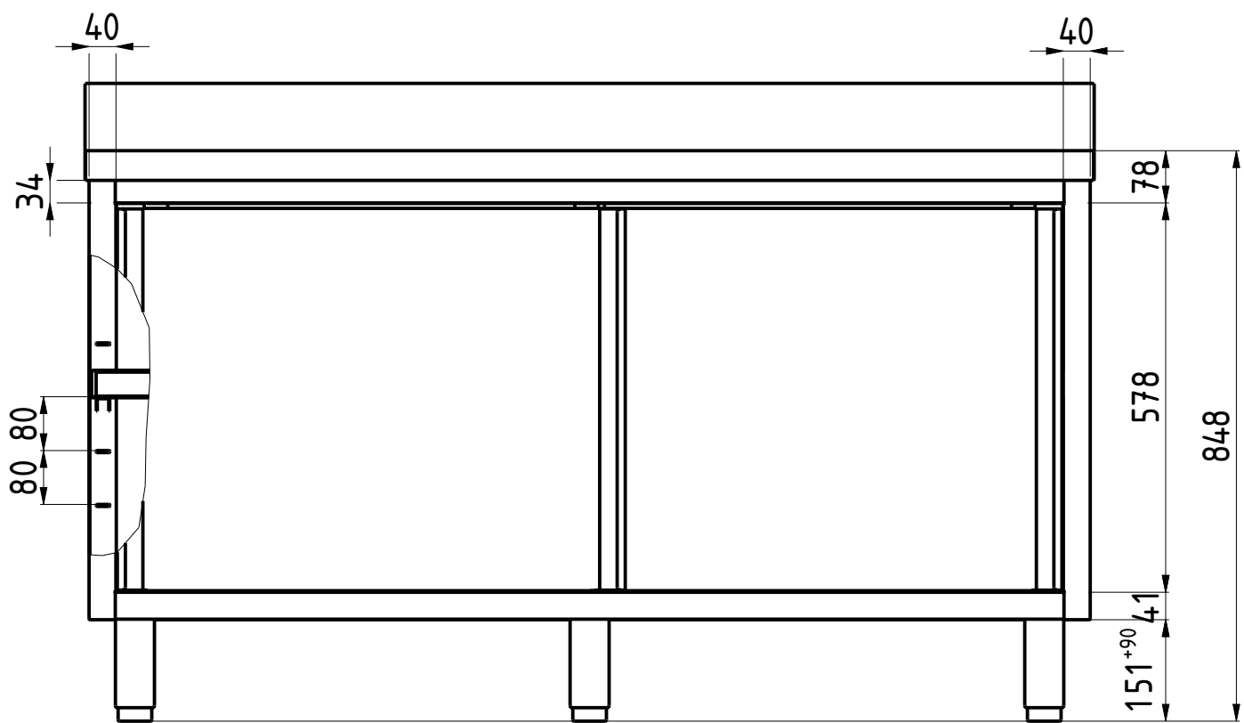
FRONT VIEW C-C 1:10
