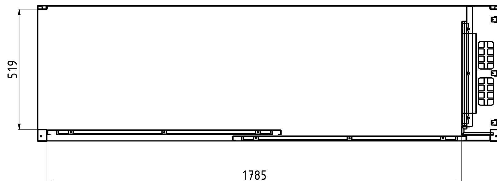
INTERNAL DIM D-D
